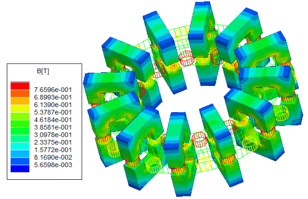
Fig. 9. The magnetic flux density in the stator cores for R_{in}=38 mm at \theta_c=0^\circ .
